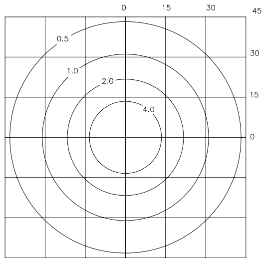
PHOTOMETRICS - ISOFOOTCANDLES 400 Watt MH @ 15' Mounting Height
